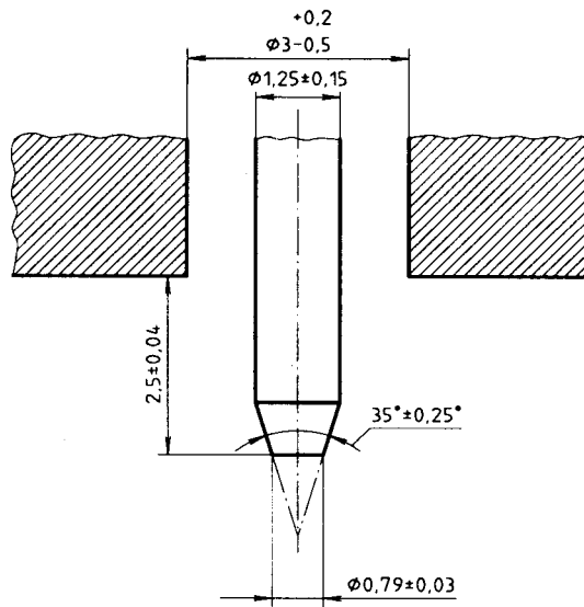
Figure 1 — Indenter for type A durometer
